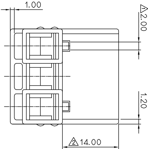
VIEW "A"
