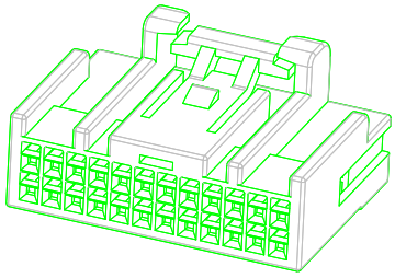
ISO VIEW
