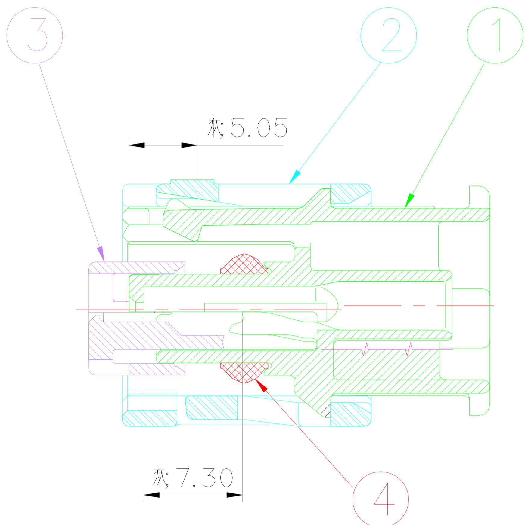
SECTION B-B
