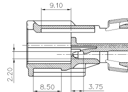
SEC B-B
