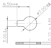
KEY HOLE PANEL DIMENSIONS
