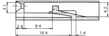
TERM' LOCK (4/1)
