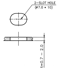
적용 BRACKET (2/1)
