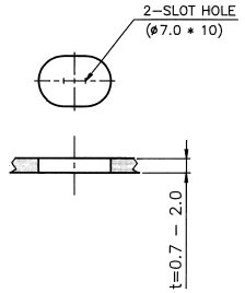
적용 BRACKET (2/1)
