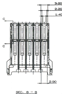
SEC. B - B
